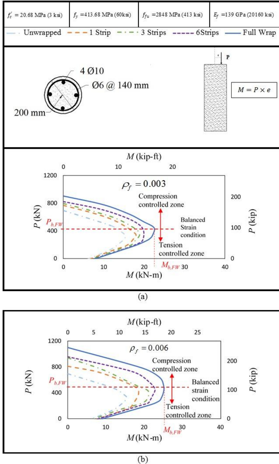
Figure 5.5 – Comparison of ( P - M ) interaction diagrams for the unwrapped column and columns having the same CFRP volumetric ratio, (a) \rho_f = 0.003 , and (b) \rho_f = 0.006
