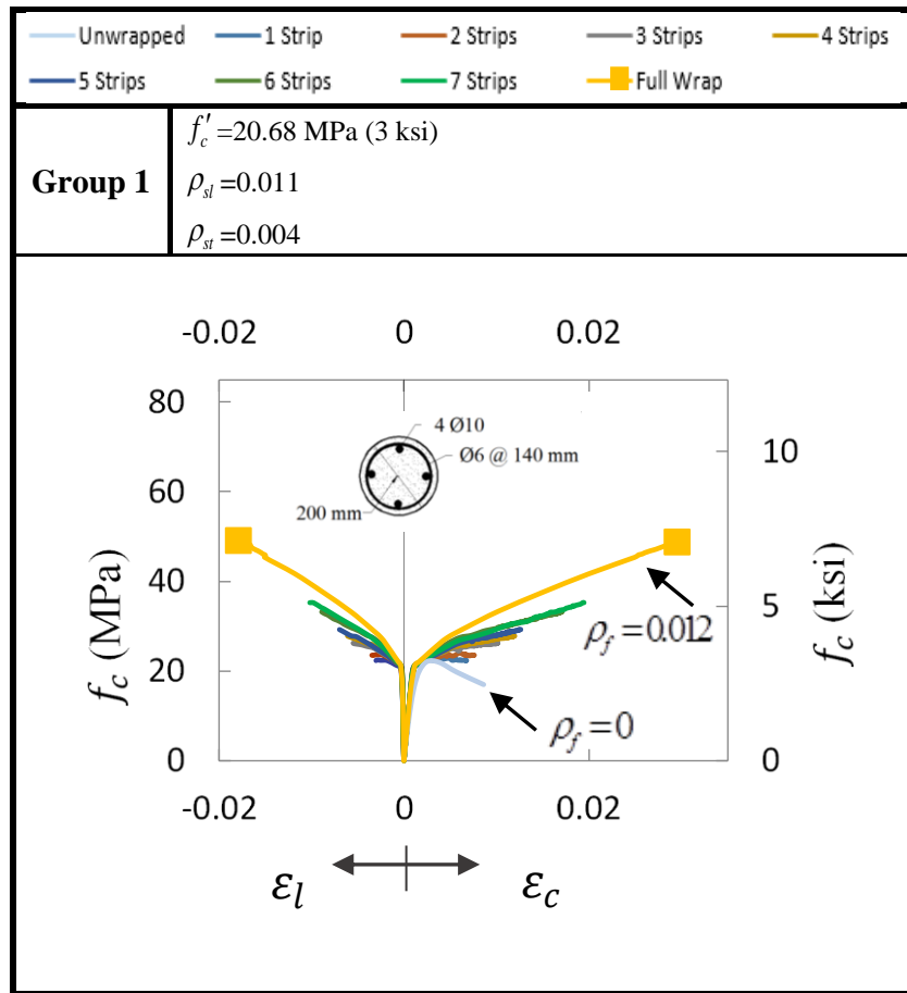
Figure 3.4- Comparison of compressive stress ( f_c ) vs axial strain ( \epsilon_c ) and lateral strain ( \epsilon_l ) for the columns in Group1 (1 mm = 0.039 in.)
