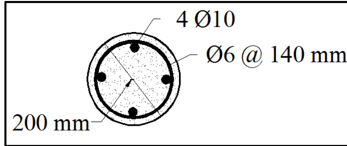
Figure 5.2– Cross sections of tested columns
